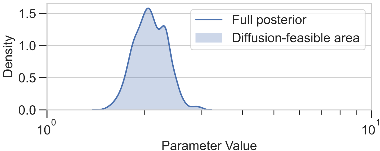
a1: Posterior with Diffusion-Feasible Area
