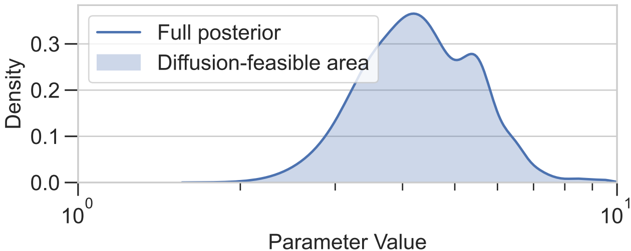
c1: Posterior with Diffusion-Feasible Area
